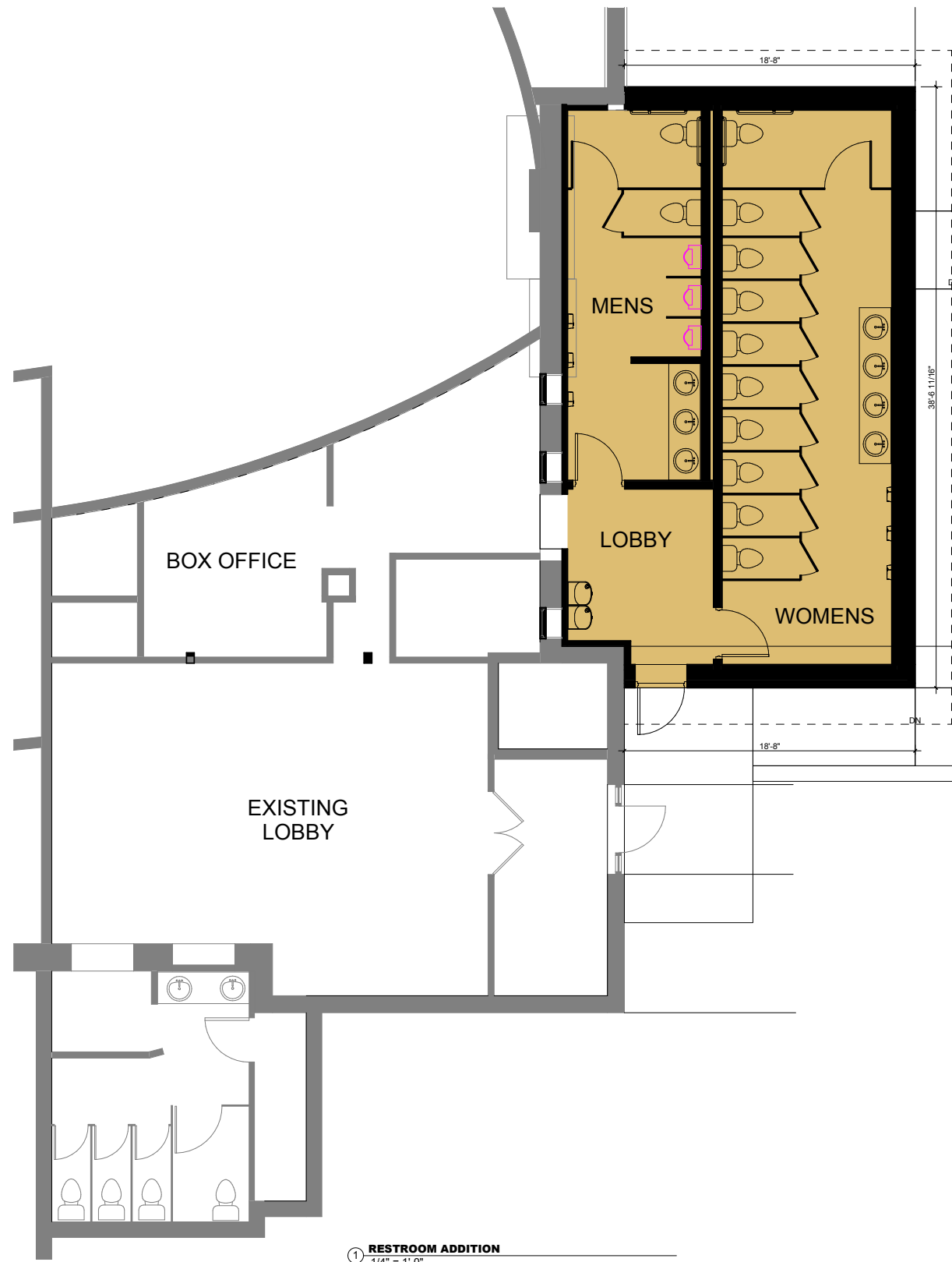
① RESTROOM ADDITION 1/4" = 1'-0"
